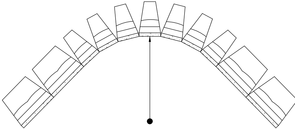
MINIMUM CONCAVE / INSIDE RADIUS FOR HALF BLOCK - PLAN VIEW
