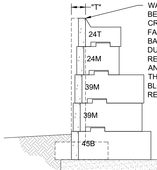
PARALLEL ABUTMENT SECTION VIEW
