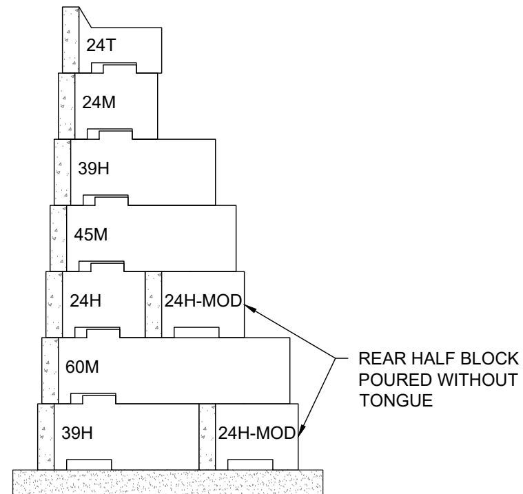
DOUBLE STACKED HALF BLOCKS - FB60 SECTION VIEW
